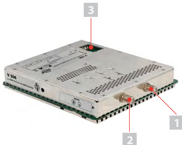
Figure 1: V 506 plug-in card
