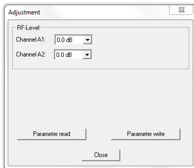
Figure 10: Setting the output level
